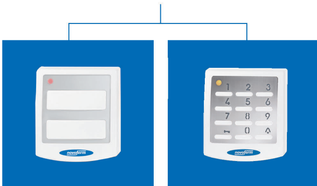
Signal 111 remote wall switch 2-channel, 433 MHz, KeeLoq rolling code for controlling 2 operators or 1 operator and 1 outside lighting in UV-resistant material
